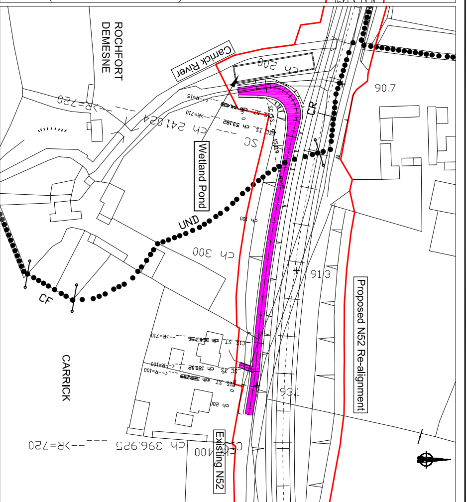
Proposed Local Access Road at Carrick
