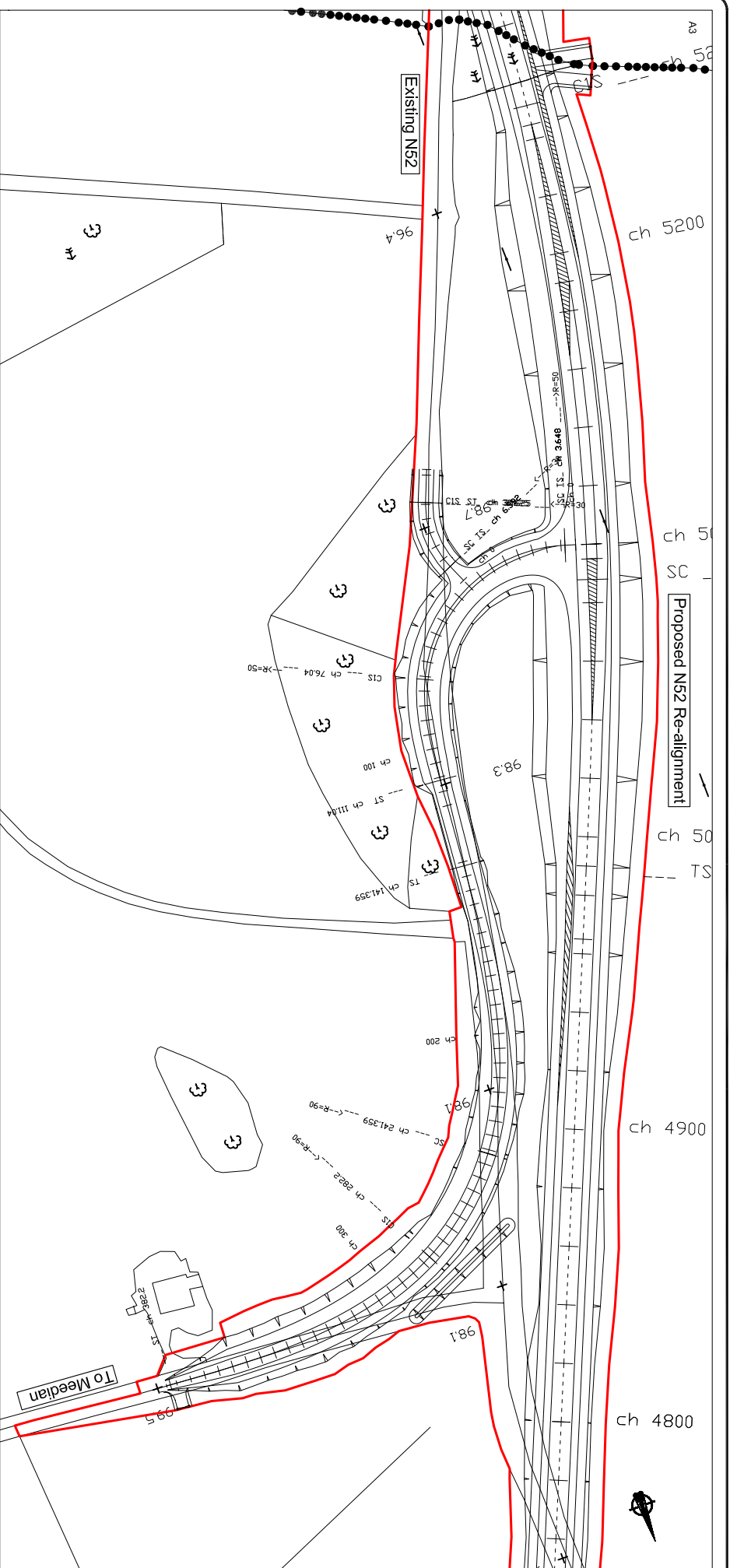
Proposed Median Road Re-alignment
